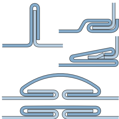
Standing seam, Pittsburgh seam, Snaplock seam
